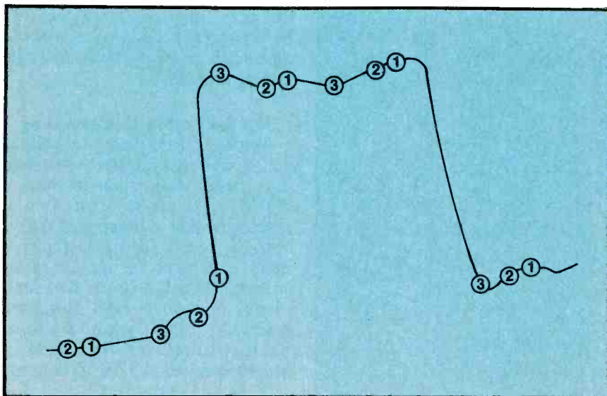
Figure 3. If the display sweep speed is slow compared to the sampling rate, a complete record of the waveform is obtained.
