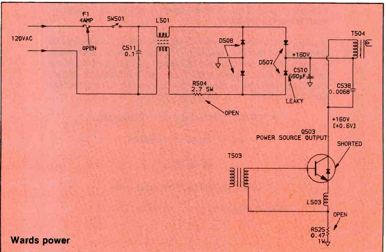
Figure 5. Five components were replaced before the power supply and power-source regulator operated correctly. Complicating the analysis was the "hot" ground that is used for all circuits shown here, as vs. the "cold" ground used for the remainder of the circuits, including the horizontal-output stage. See the text for details.
