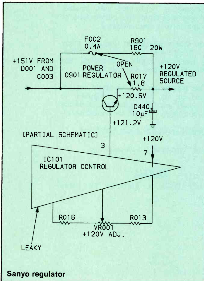
Figure 3. One component failed and that started a chain reaction requiring four new components in the Sanyo power-regulator circuit.
