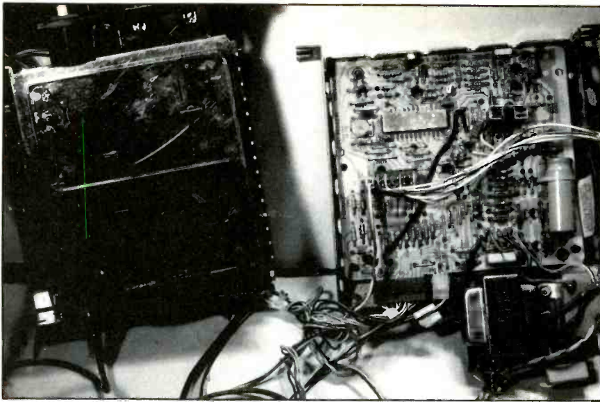
Often the tuners and the control module are fastened together and mounted upright beside the horizontal TV chassis. A cable connects them to the chassis. The control module turns on the TV power via a relay and controls many TV functions.
