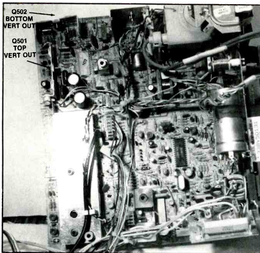
Arrows point to Q502, the bottom vertical output transistor, on its heat-sink in the upper left corner of the photograph, and to Q501, the top vertical output transistor, on another heat-sink just below Q502 (in the photograph). This is an RCA CTC120 chassis.
