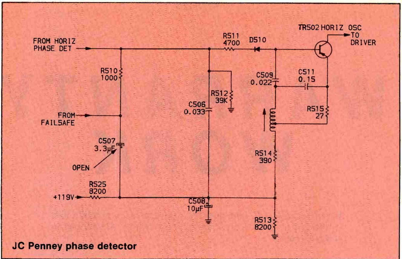
Figure 4. A dried-out C507 electrolytic in the JC Penny horizontal phase detector circuit caused pie-crusting. C507, in series with 1,000Ω R510 formed a long time constant to keep the control voltage constant over one vertical field (approximately).
