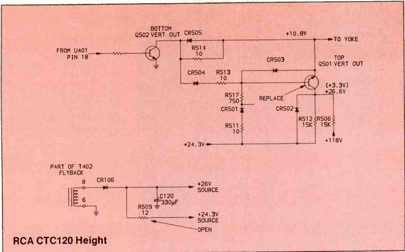
Figure 1. A loss of the +24.3V source voltage eliminated the vertical sweep and reduced the dc voltages at Q502 and Q501. An open 12Ω R509 in the power supply was responsible. The original defect was a malfunctioning tuner-control module that refused to activate the power on/off relay in this RCA CTC120 receiver.
